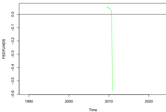
Figure 15: \phi_{FEDFUNDS}^{RSM}
