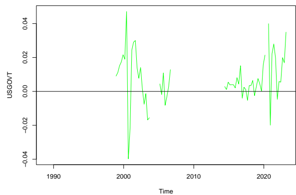
Figure 16: \phi_{USGOVT}^{RSM}
